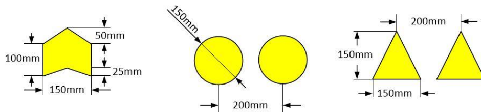
Figure 30 - 2013 Section Isolator Marks Dimensions
