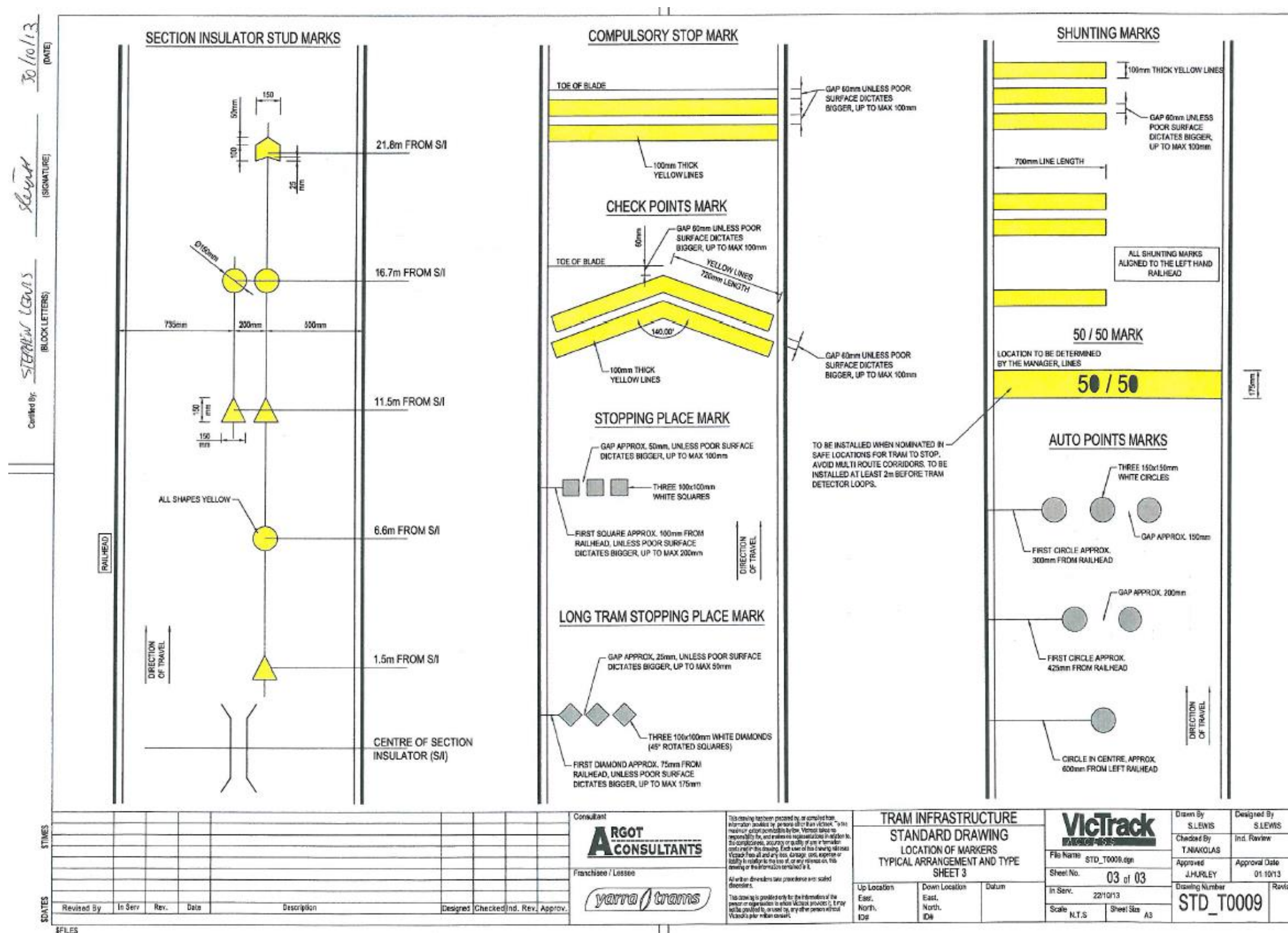
Figure 37 - Standard Drawing Location of Markers Typical Arrange and Type STD_T0009 3 of 3
