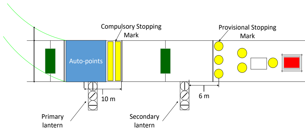
Figure 6 - Example of Tram Signal Lantern Installation
