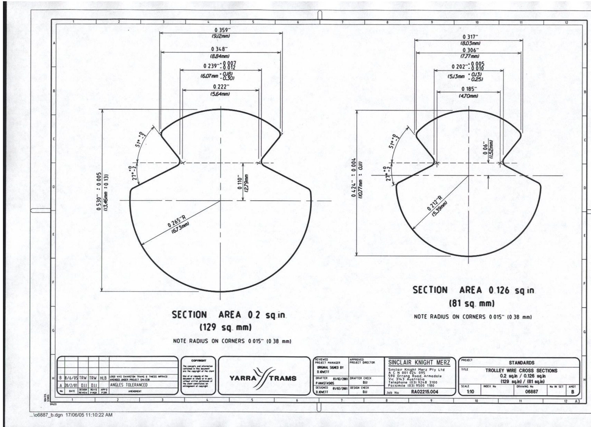
Figure 1. Drawing O6887 Rev.B for 0.2 sq.in. trolley wire (129mm 2 ) and 0.126 sq.in. trolley wire (81 mm 2 )
