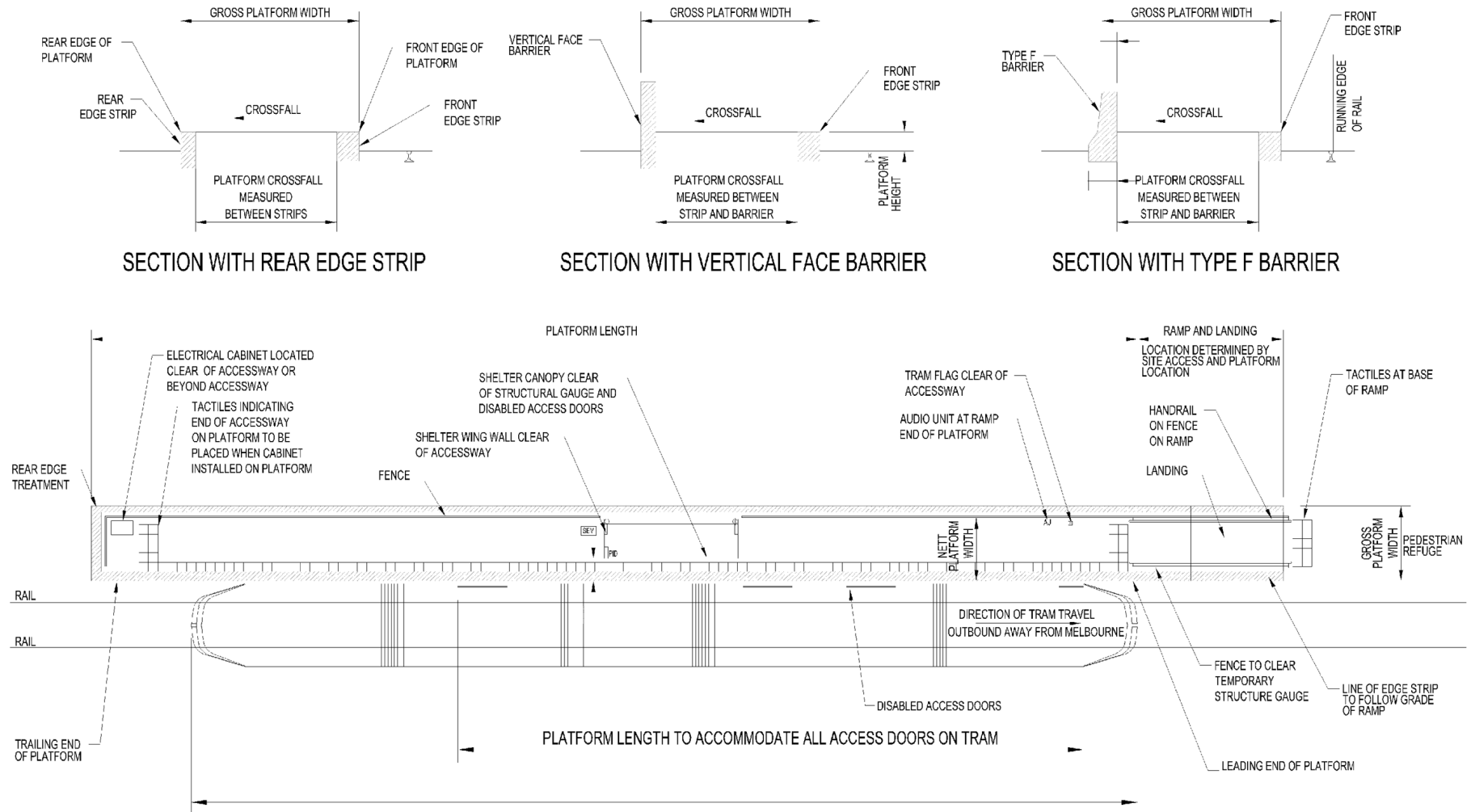
FEATURES OF ACCESSIBLE TRAM STOP - TYPICAL ARRIVAL STOP
