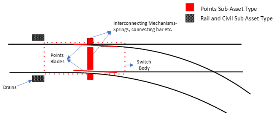
Figure 1 - Manual Facing Points, Springloaded Points and Trailing Points
